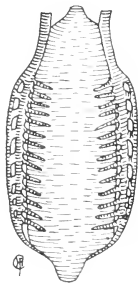
Fig. 21. Rectal tracheae of dragonfly.
